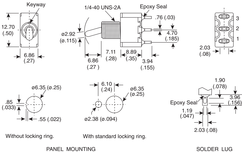
PANEL MOUNTING
